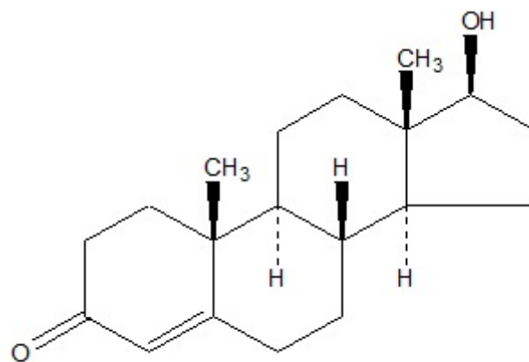
Testosterone
